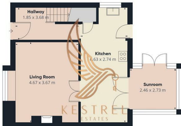
Floor 0 Building 1
