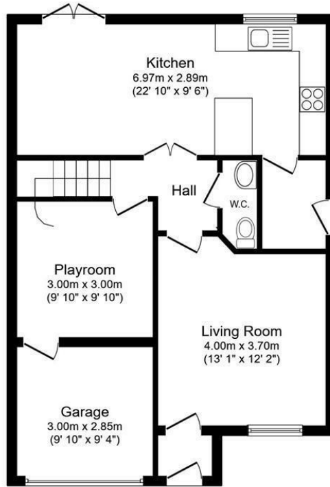
Ground Floor Floor area 67.7 m 2 (729 sq.ft.)
