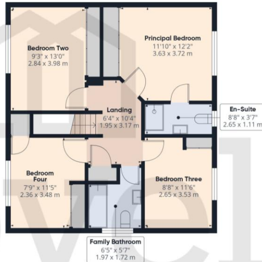
Floor 1 Building 1
