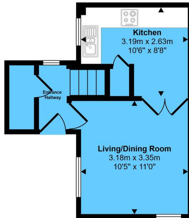
Ground Floor Approx 24 sq m / 254 sq ft
