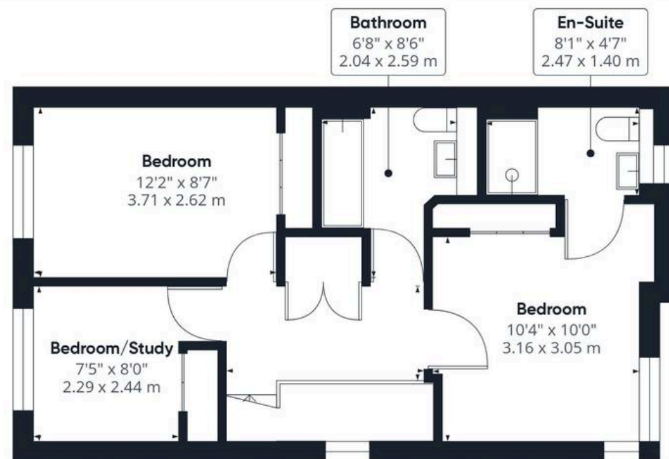
Floor 1
