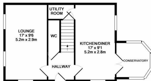
GROUND FLOOR APPROX. FLOOR AREA 475 SQ.FT. (44.1 SQ.M.)
