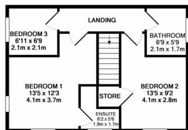
1ST FLOOR APPROX. FLOOR AREA 416 SQ.FT. (38.7 SQ.M.)
