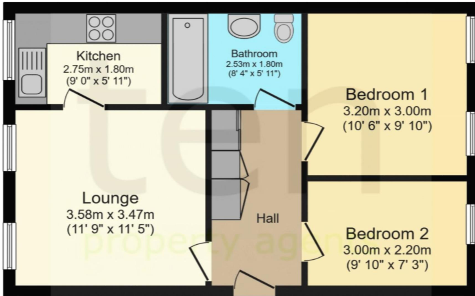
Floor Plan
