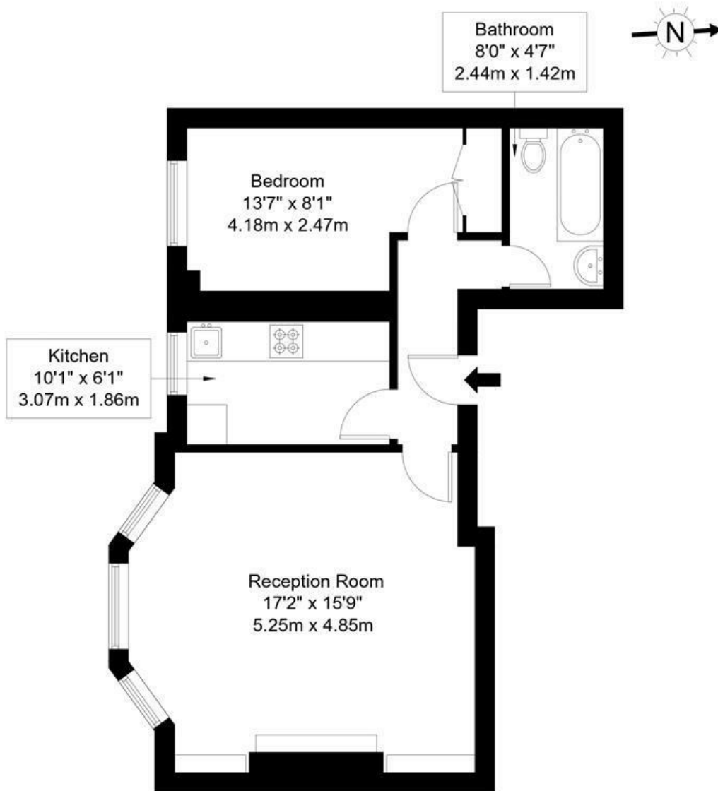
First Floor
