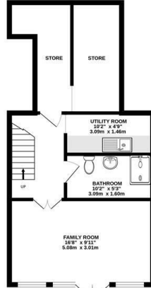
BASEMENT 471 sq.ft (43.9 sq.m) approx.
