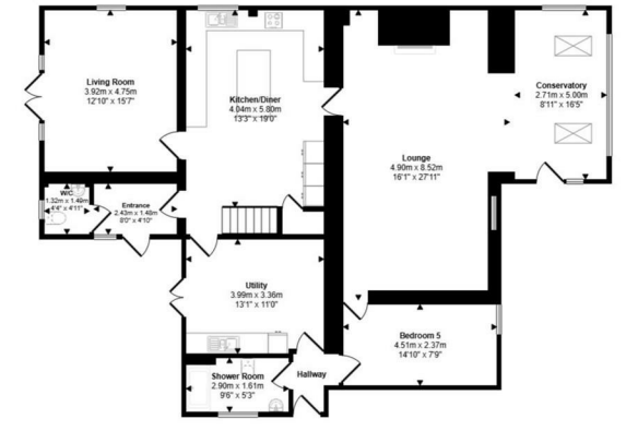
Ground Floor Approx 147 sq m / 1588 sq ft
