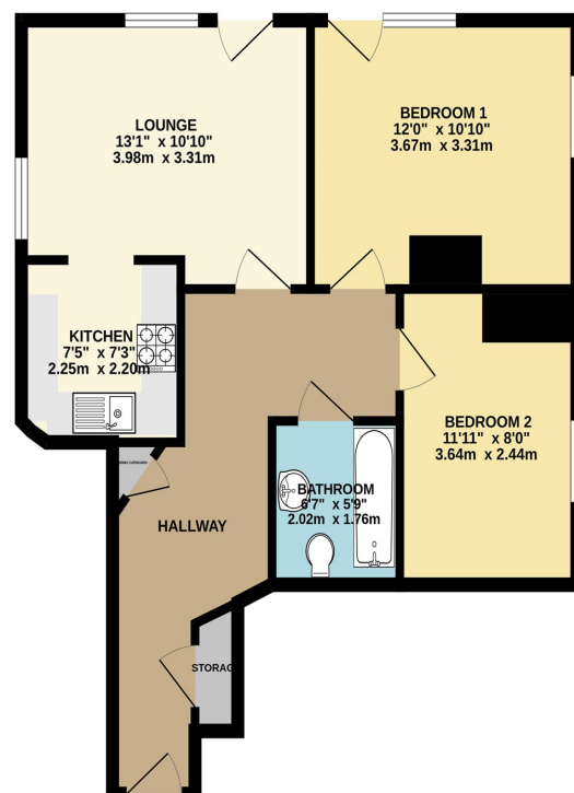
TOP FLOOR
