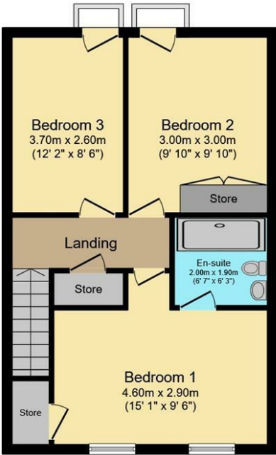
Second Floor Floor area 48.3 sq.m. (520 sq.ft.)
