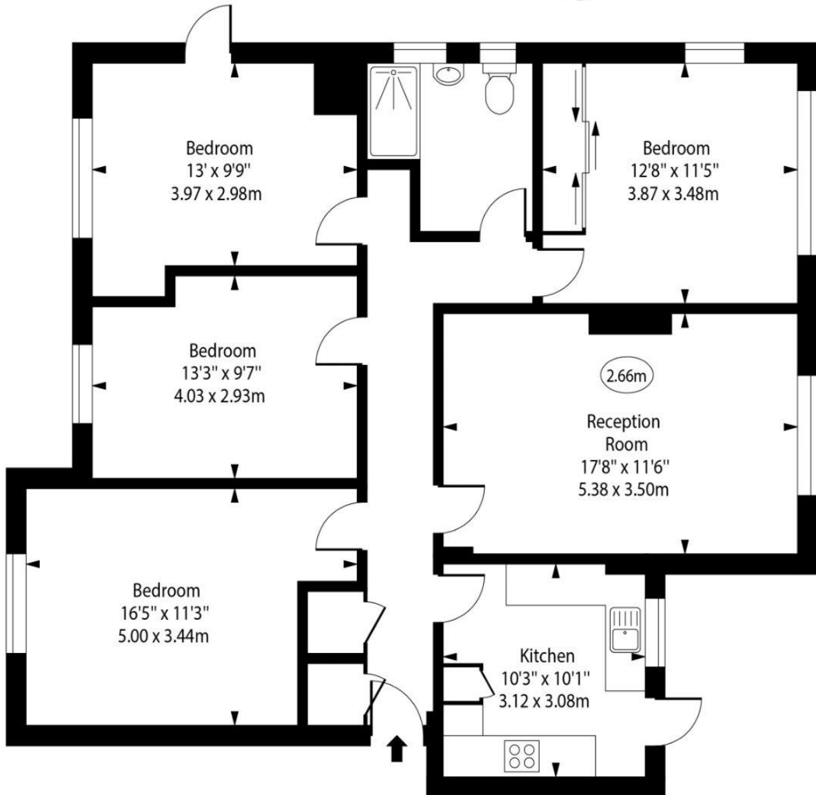
Ground Floor
