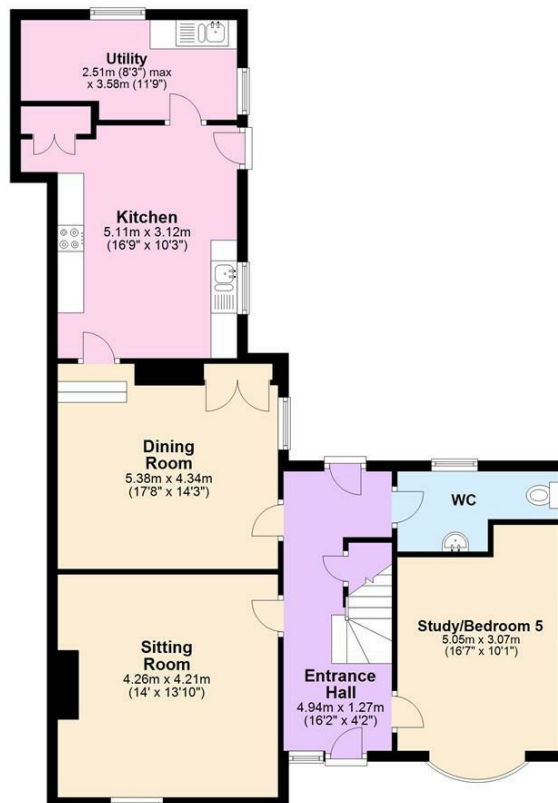
Ground Floor Approx. 95.5 sq. metres (1027.5 sq. feet)
