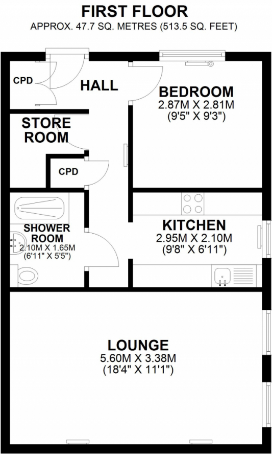
TOTAL AREA: APPROX. 47.7 SQ. METRES (513.5 SQ. FEET)
