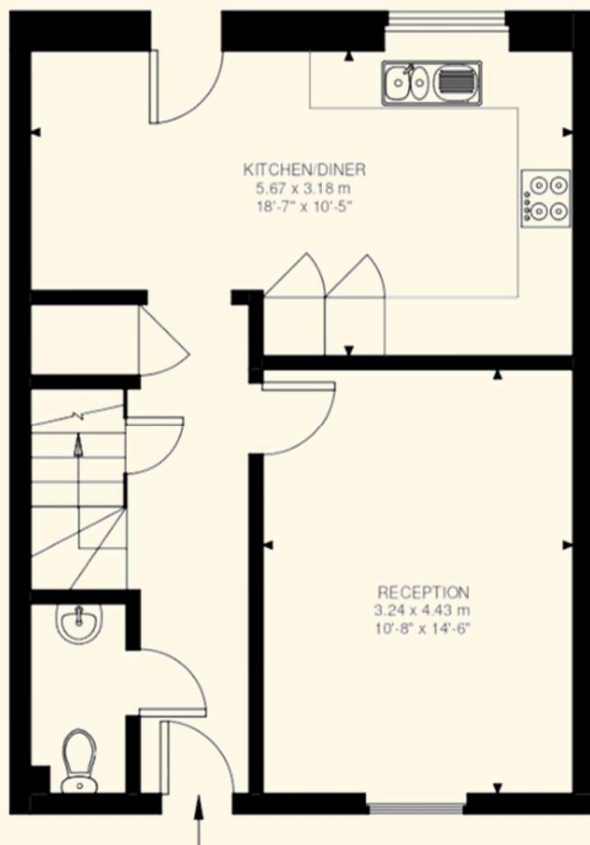
Ground Floor 476 ft²
