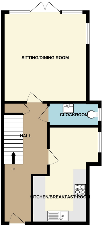
GROUND FLOOR 483 sq.ft. (44.8 sq.m.) approx.
