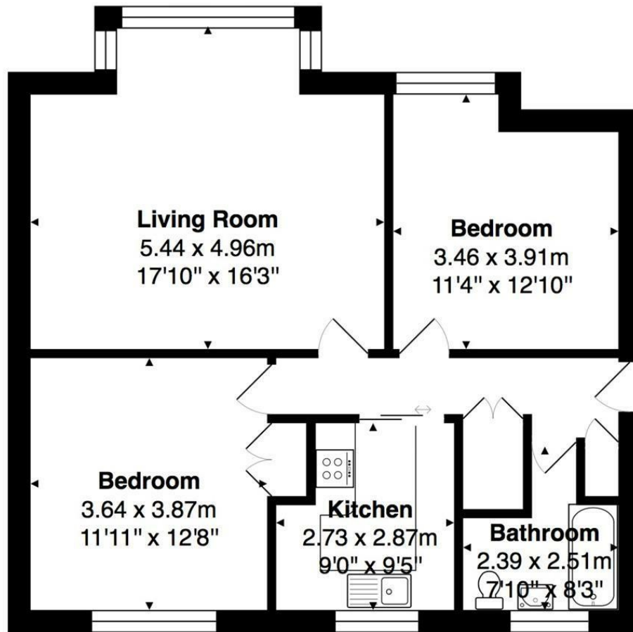
Third Floor Area: 73.3 m 2 ... 789 ft 2
