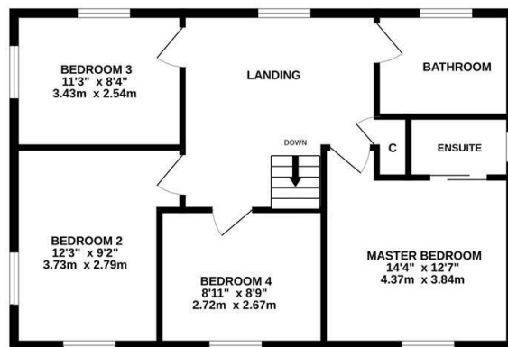
1ST FLOOR 653 sq.ft. (60.7 sq.m.) approx.
