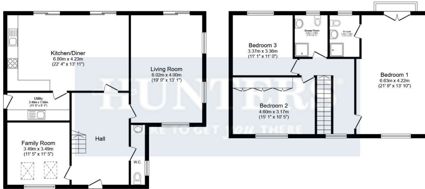
Ground Floor Floor area 92.3 sq.m. (993 sq.ft.)
