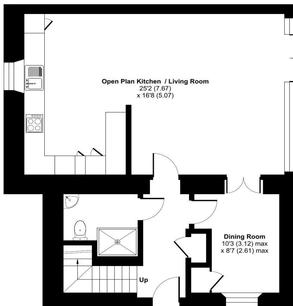
GROUND FLOOR
