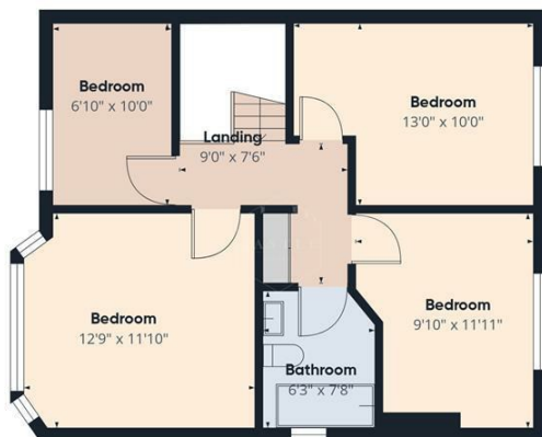
Floor 1 Building 1
