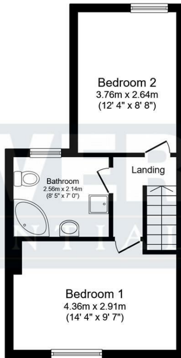
First Floor Floor area 32.6 sq.m. (351 sq.ft.)
