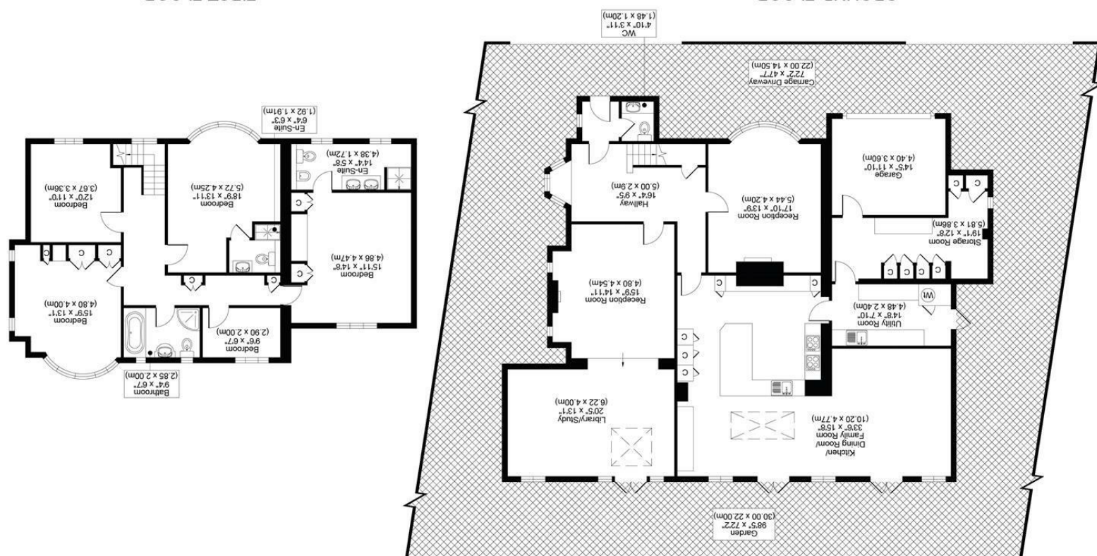
FIRST FLOOR
