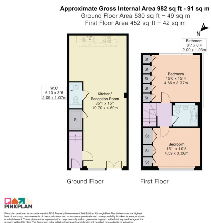
Floor Plan
