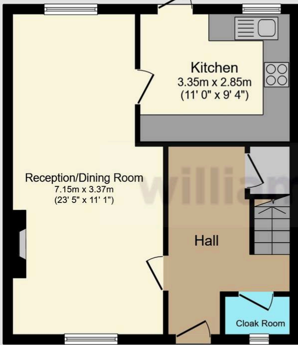
Ground Floor Floor area 44.3 sq.m. (477 sq.ft.)
