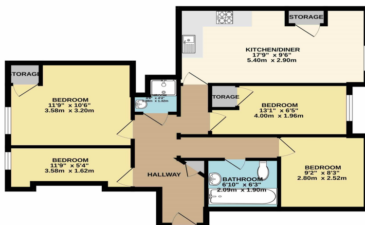
THIRD FLOOR
