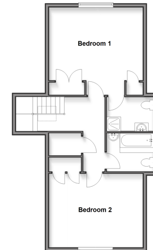
First Floor Approx. 60.1 sq. metres (646.5 sq. feet)
