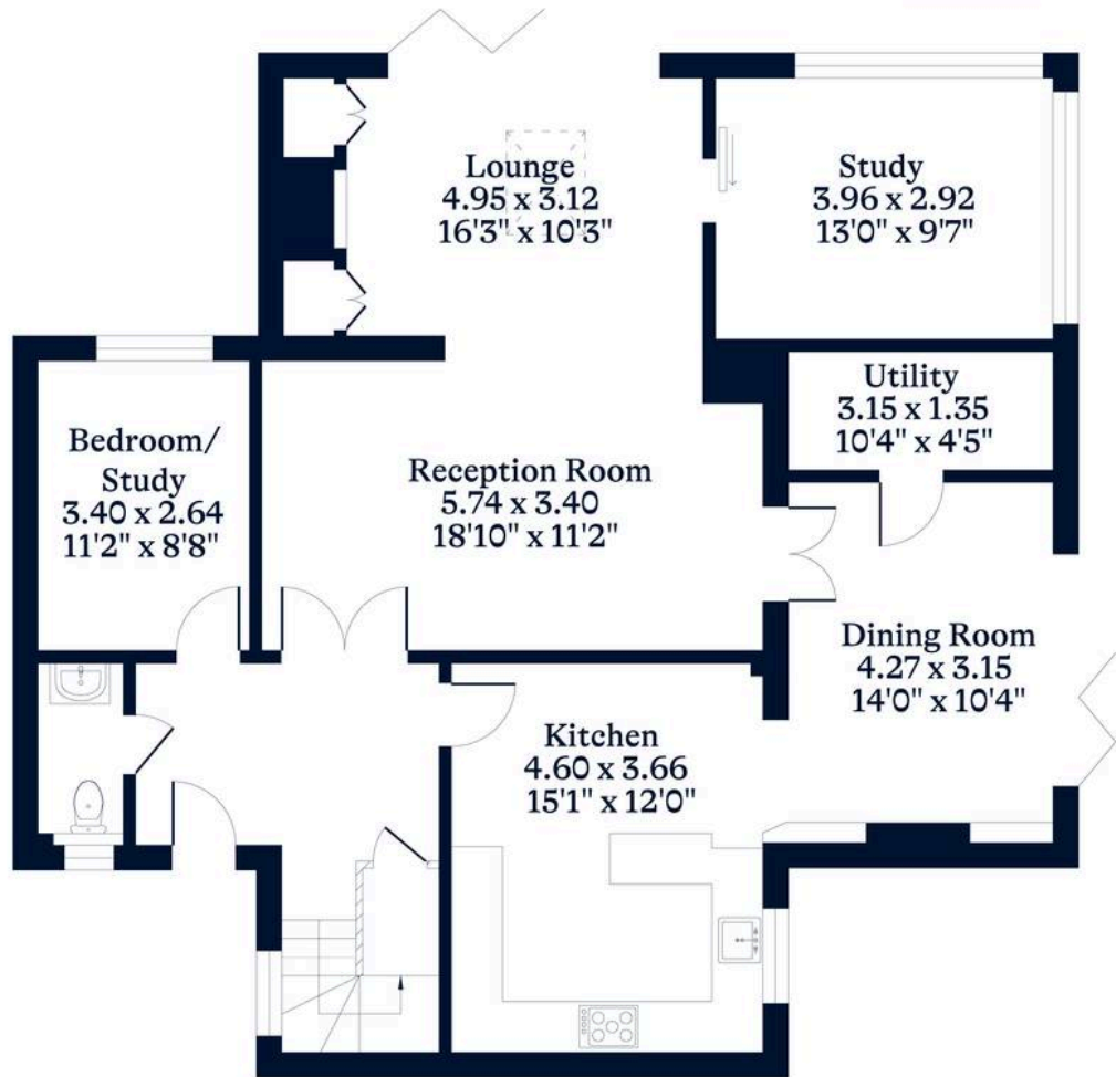
Ground Floor
