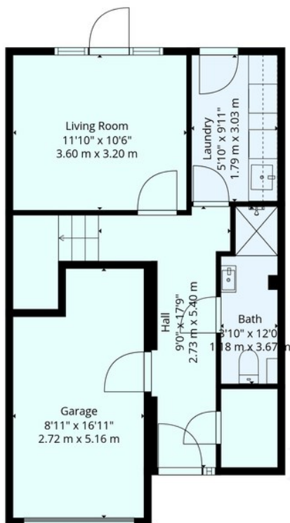
Floor 1
