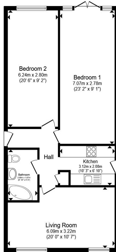
Floor Plan
