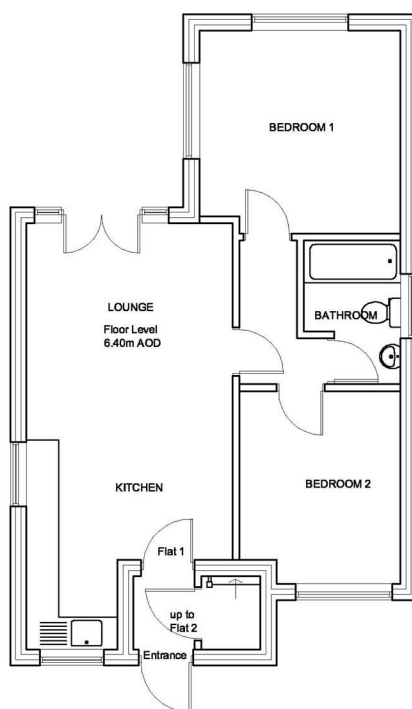
GROUND FLOOR PLAN 1:100
