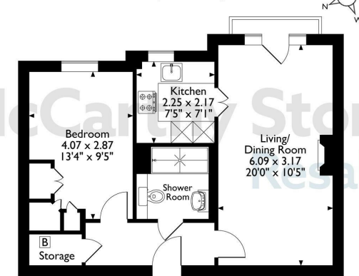
Ground Floor Flat
