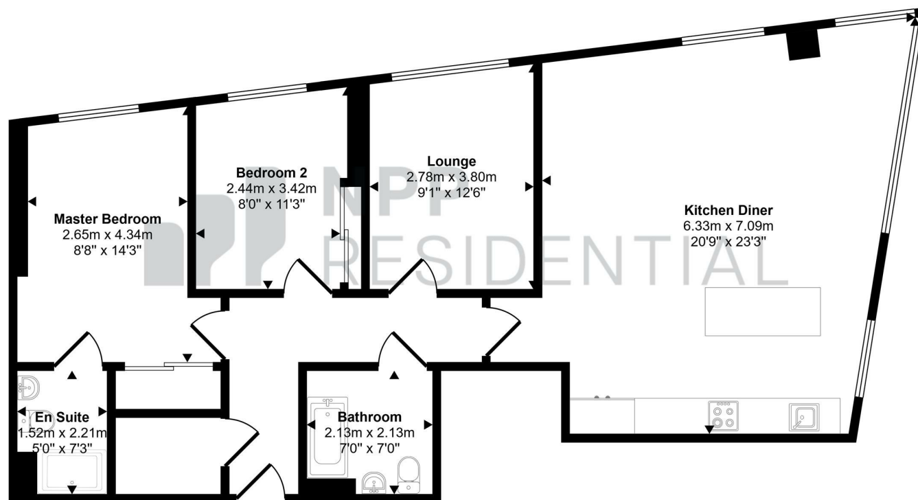
Floorplan
