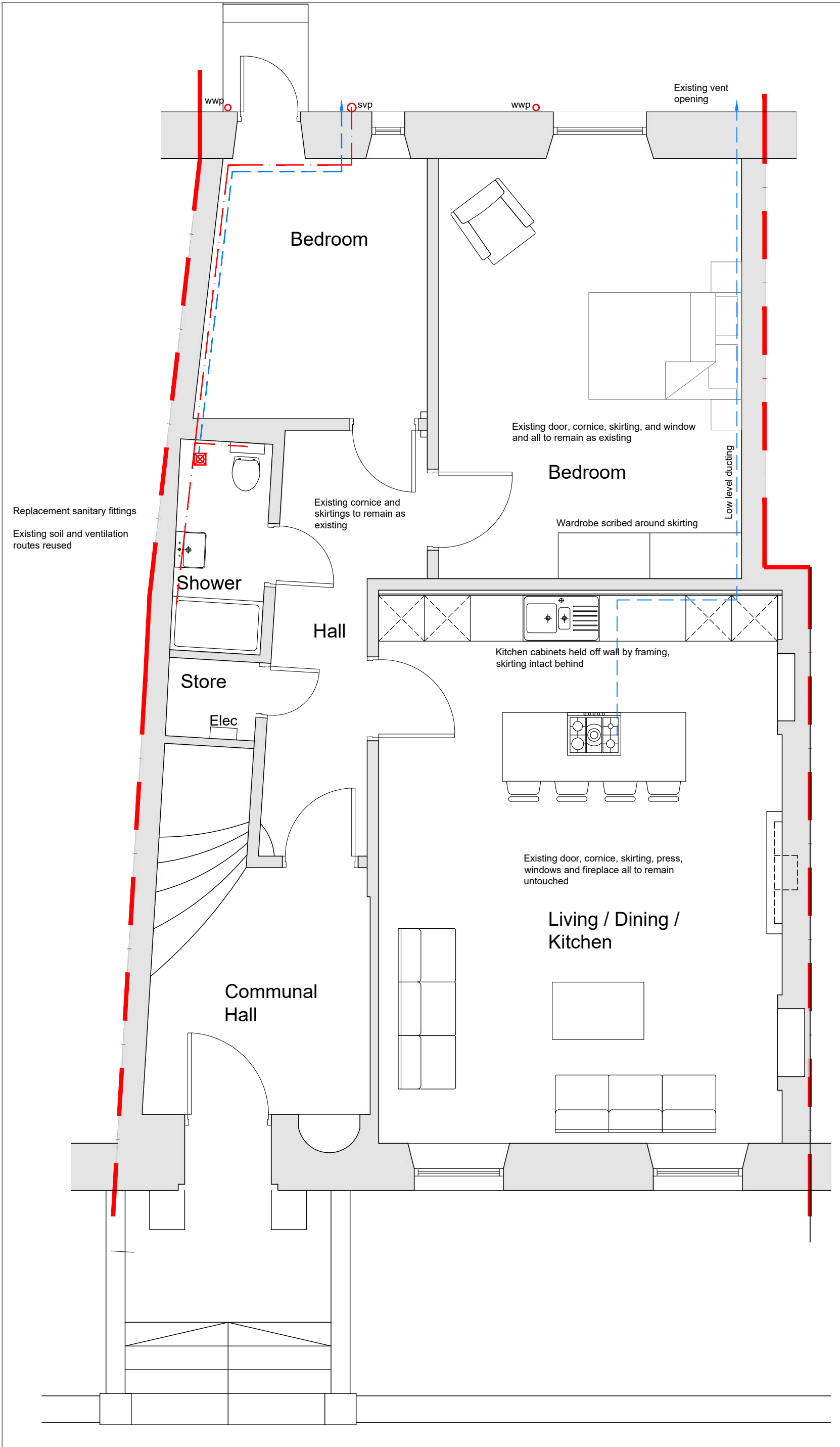
PROPOSED GROUND FLOOR PLAN - 1:50 @A3
