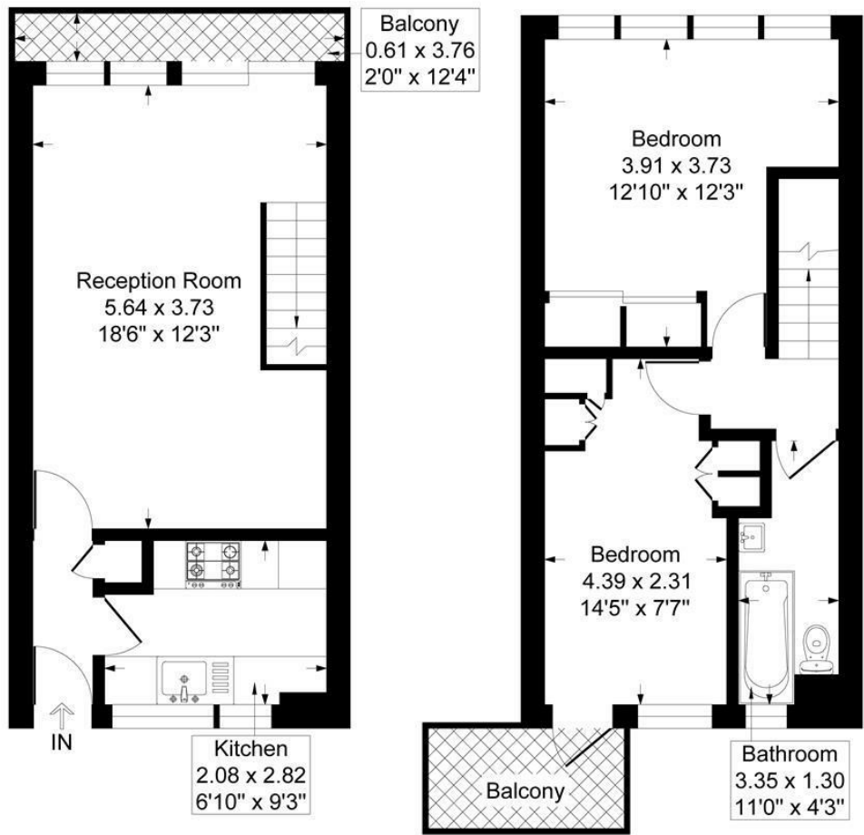
Third Floor
