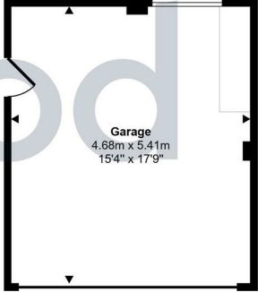
Garage Approx 25 sq m / 273 sq ft
