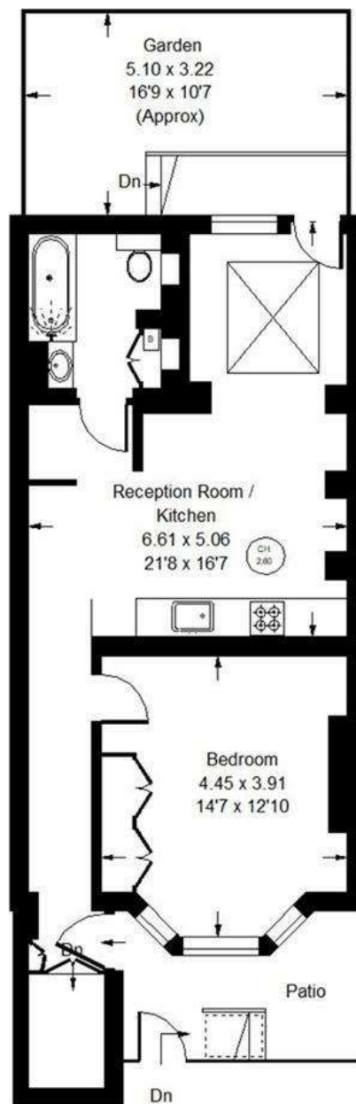
Ground Floor
