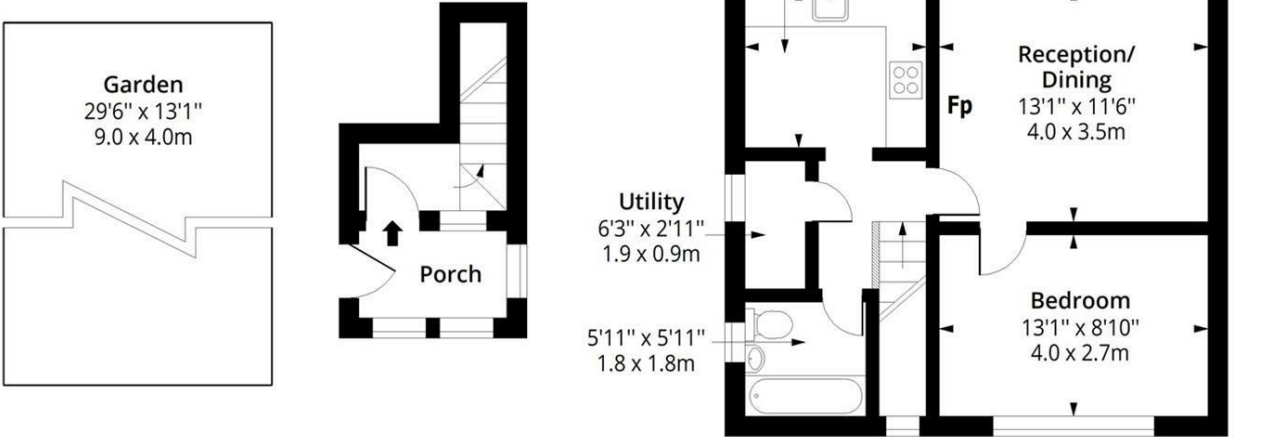
Ground Floor Floor Area 75 Sq Ft - 6.97 Sq M
