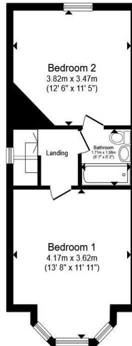
First Floor
