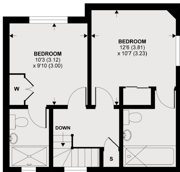
1st Floor
