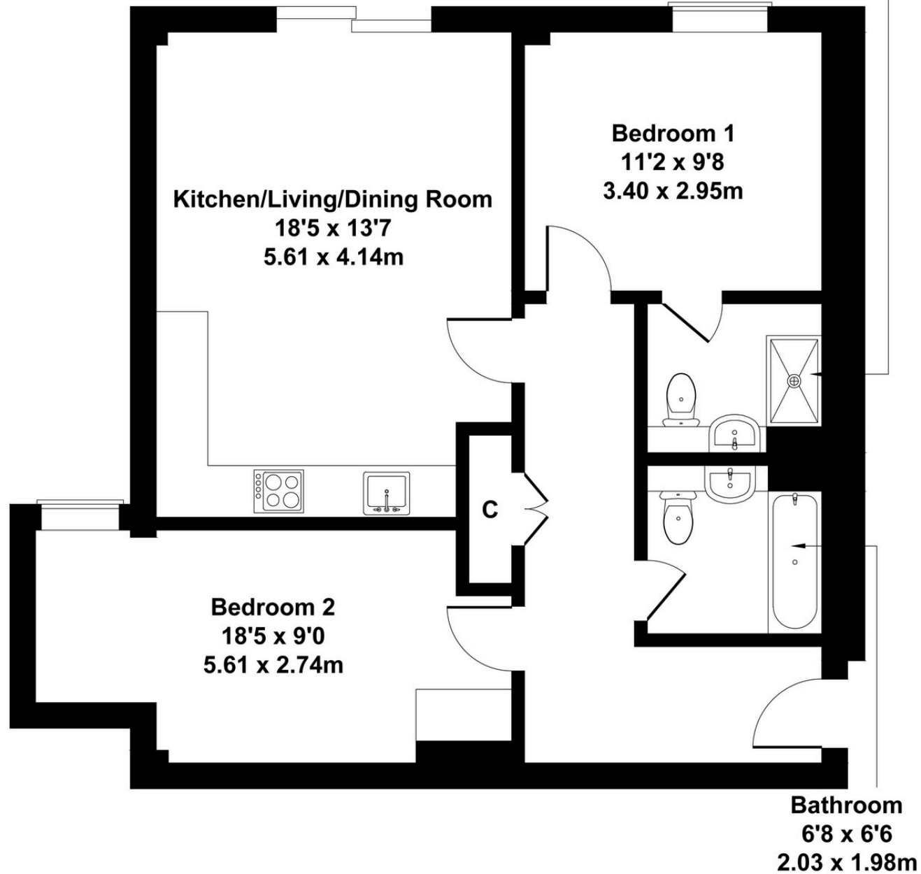
Floorplan for Flats 15, 16 & 19 Junction Court
