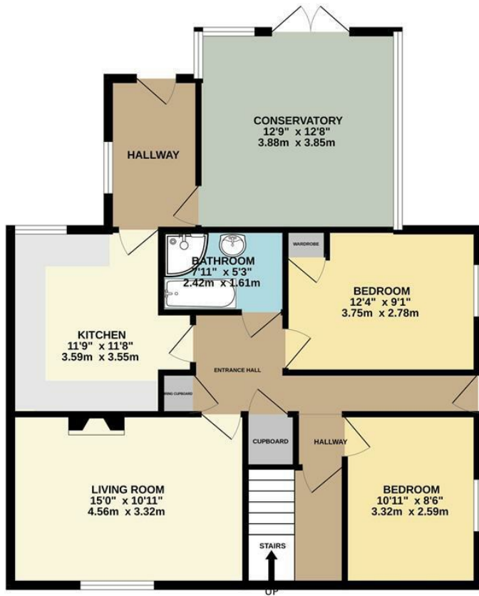
GROUND FLOOR 888 sq.ft. (82.5 sq.m.) approx.
