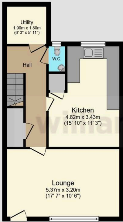
Ground Floor Floor area 47.7 sq.m. (513 sq.ft.)
