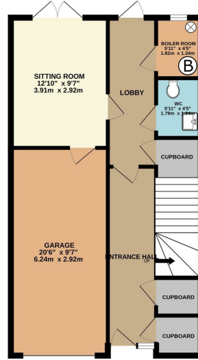
GROUND FLOOR 619 sq.ft. (57.5 sq.m.) approx.
