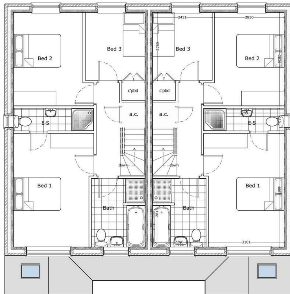
Proposed First Floor Plans
