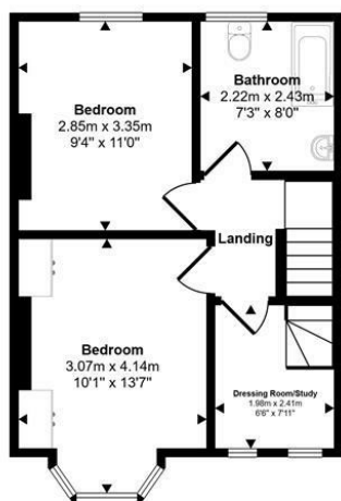
First Floor Approx 37 sq m / 402 sq ft
