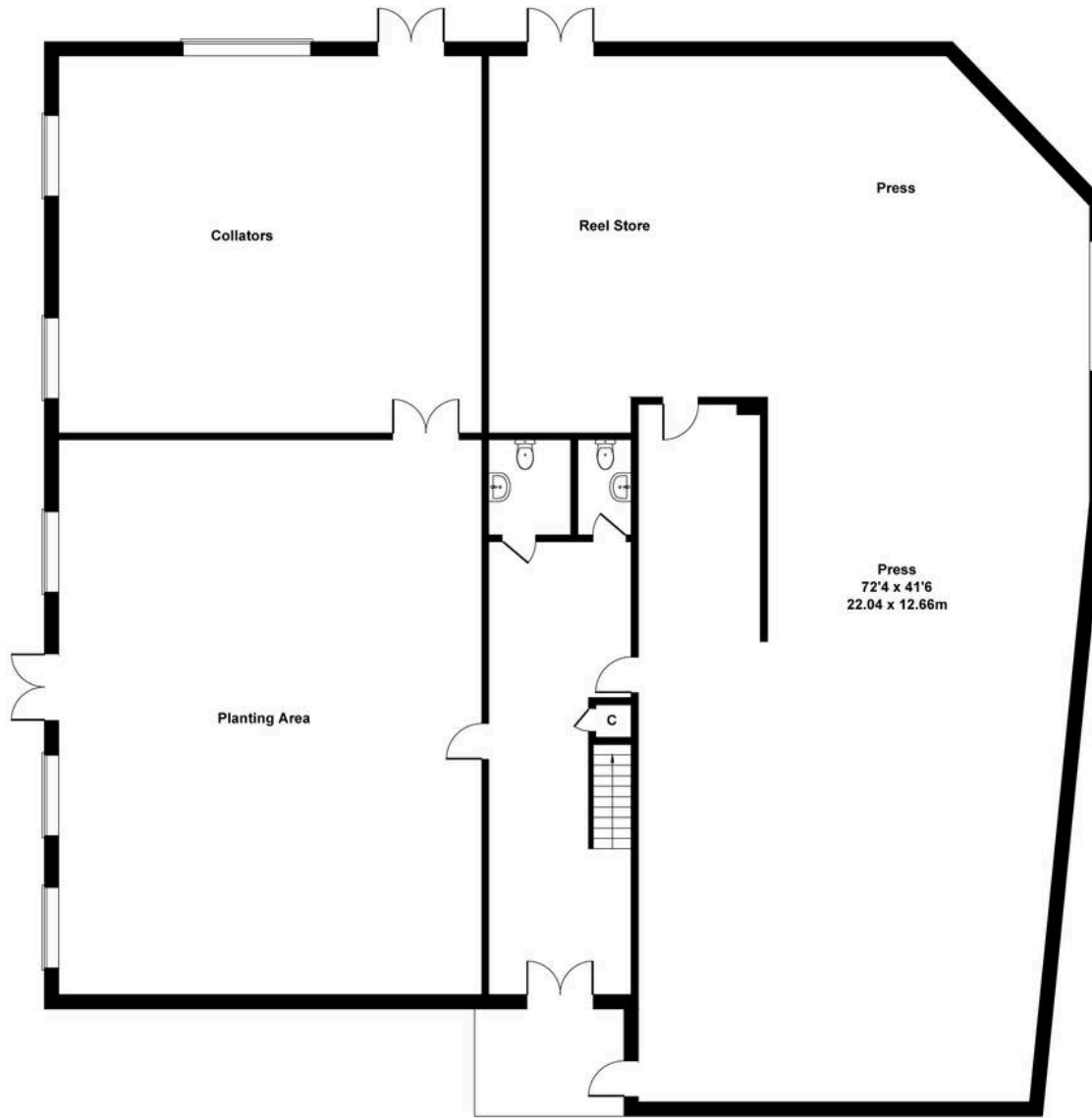
GROUND FLOOR
