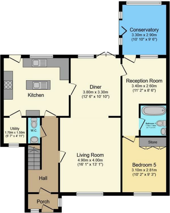
Ground Floor Floor area 101.4 sq.m. (1,091 sq.ft.)
