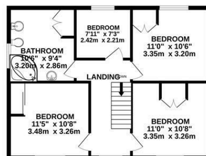
1ST FLOOR 600 sq.ft. (55.7 sq.m.) approx.
